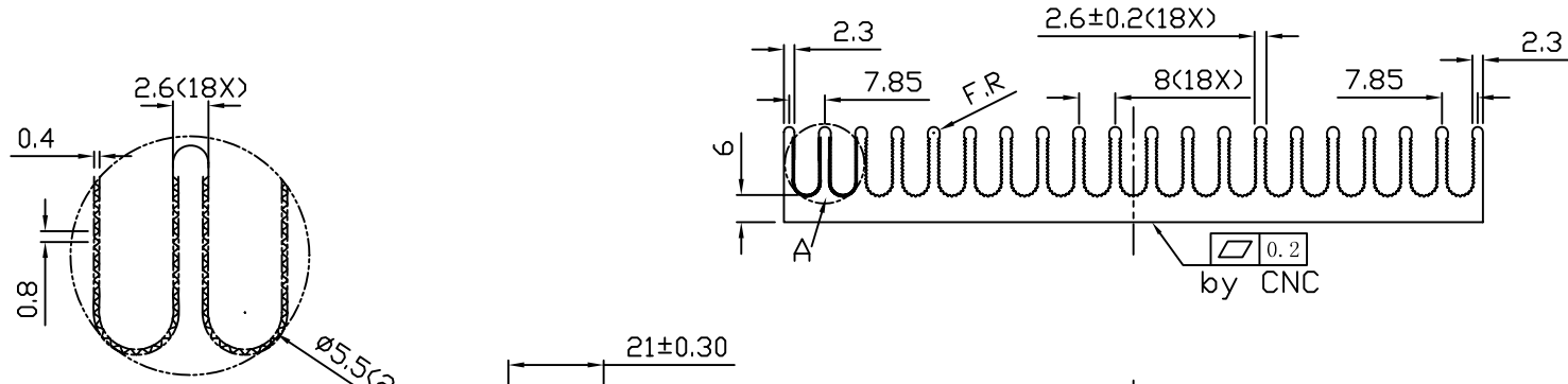
DETAIL A SCALE 3:1
