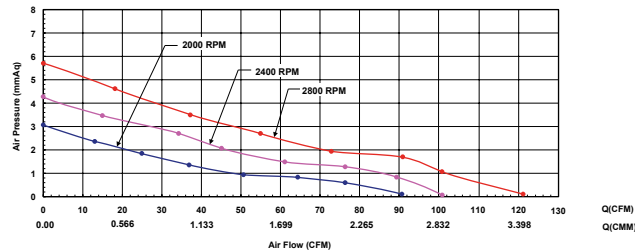
Performance curve
