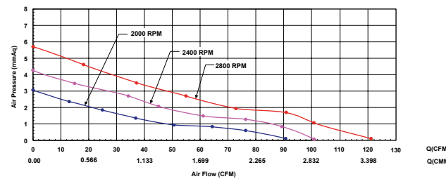
Performance curve
