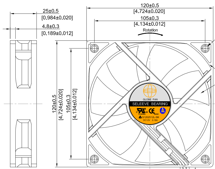
Housing drawing (SCALE :1.5:1)
