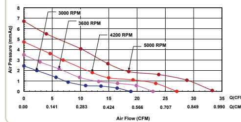
Performance curve
